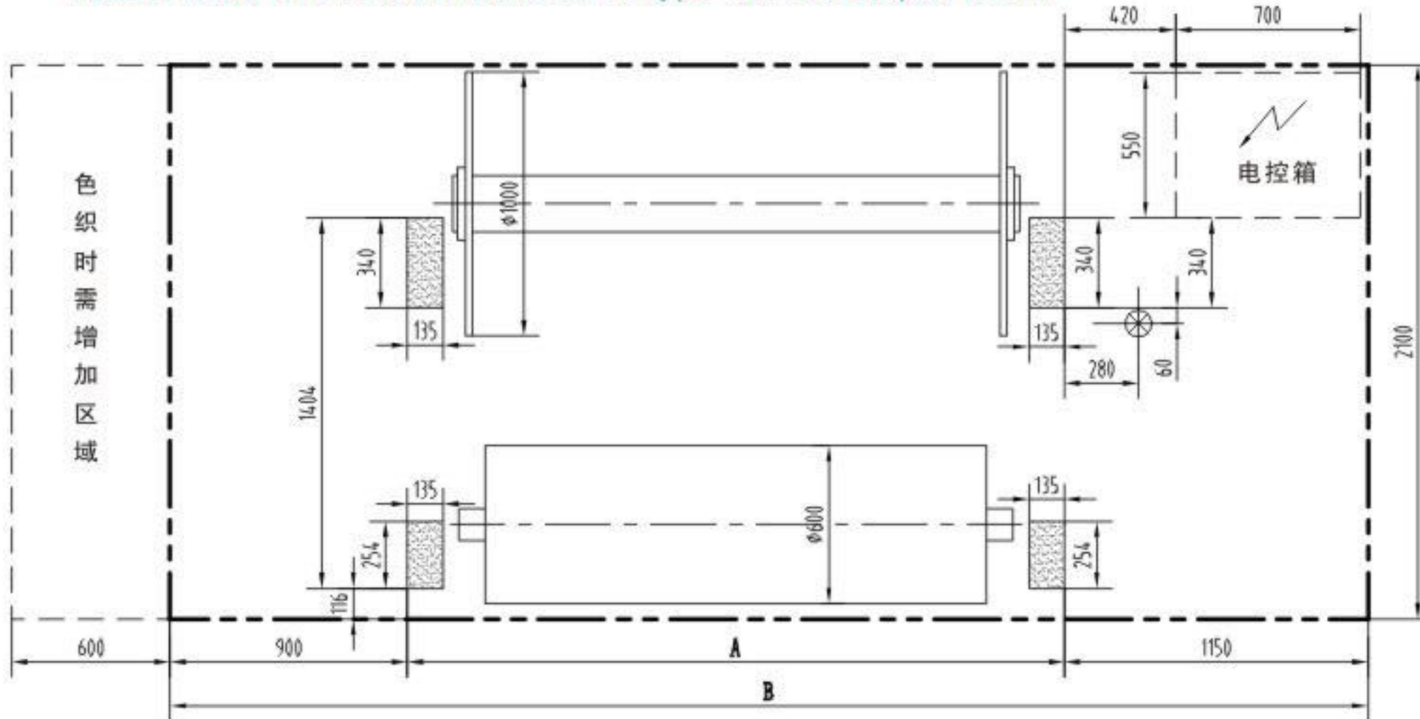
机器外形尺寸/Overall Dimension of Type G1736C Rapier Loom
